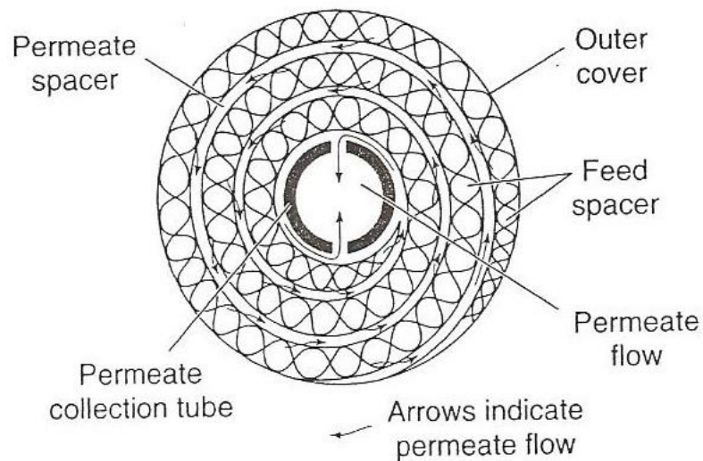
Spiral-Wound Module Cross Section
